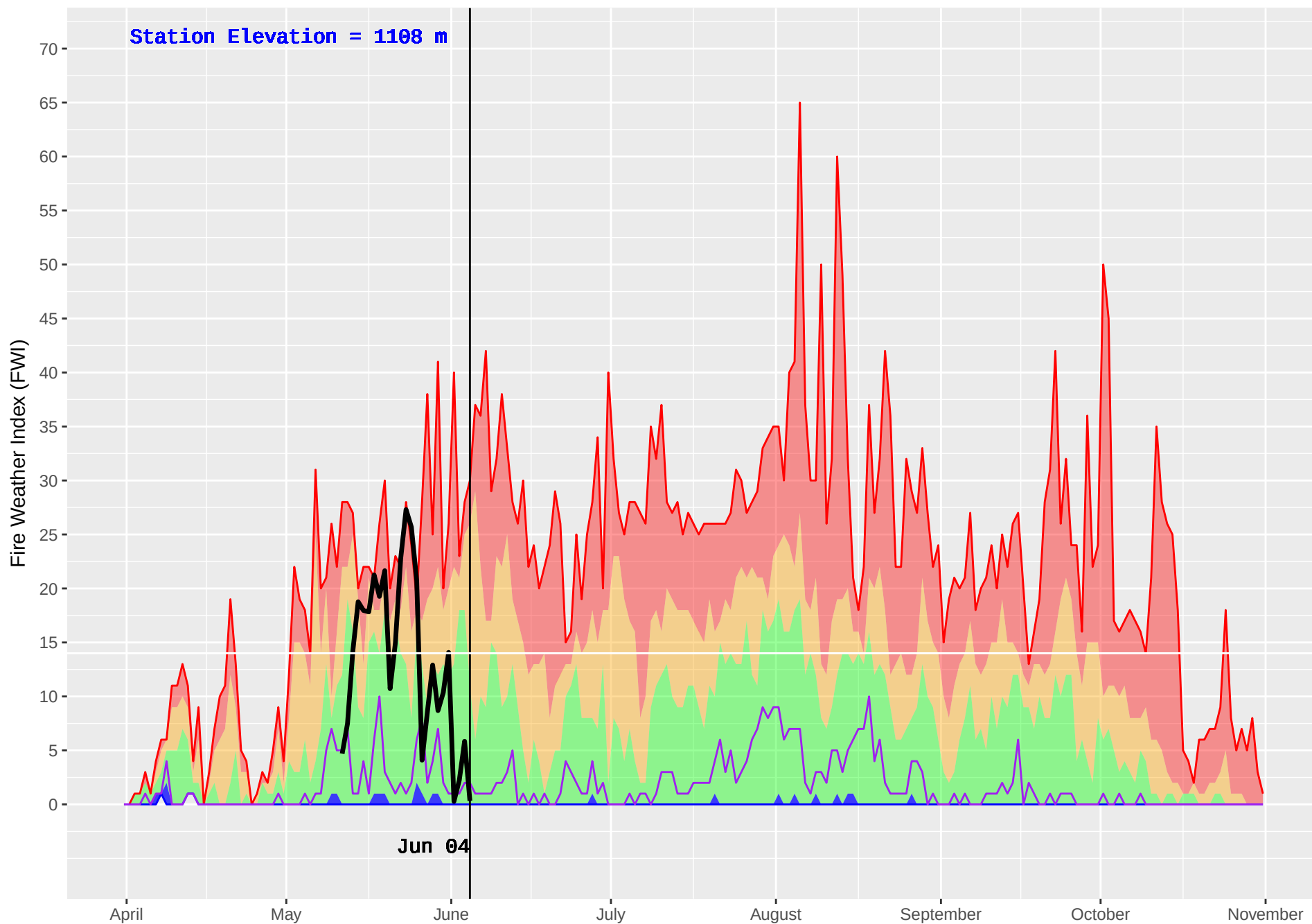
MATHEW (263) : Historical (1987–2016) and Current (2018) Noon Fire Weather Index (FWI)
